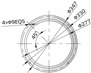
SLHR-36U-96U-S mounting base
