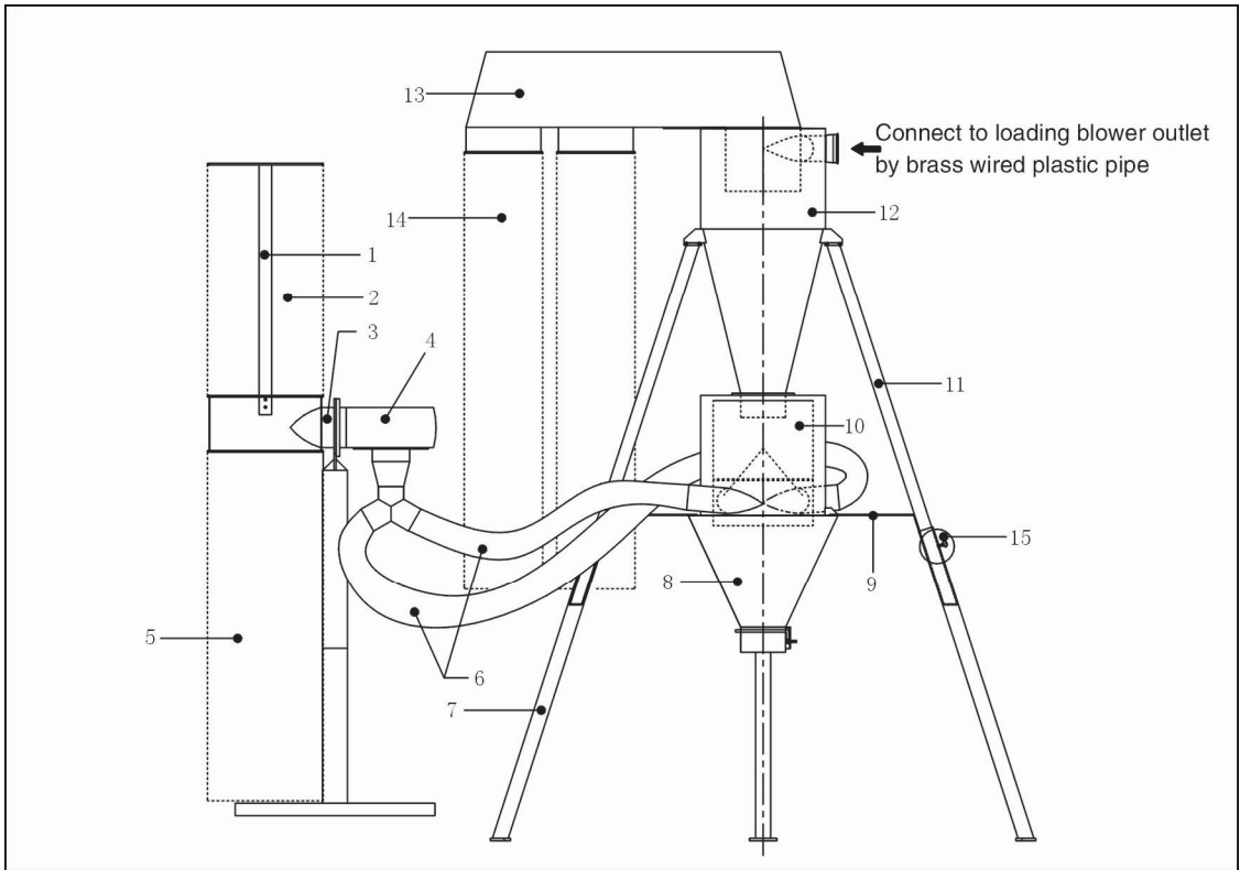
Picture 2-12: Cyclone and Dust Remove Device
