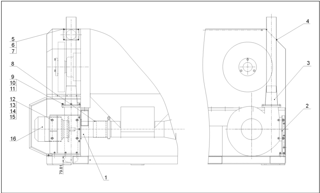
Picture 2-10: Blower
