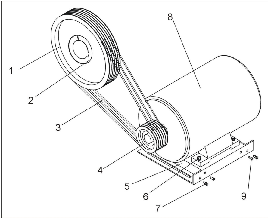
Picture 2-8: Transmission Parts
