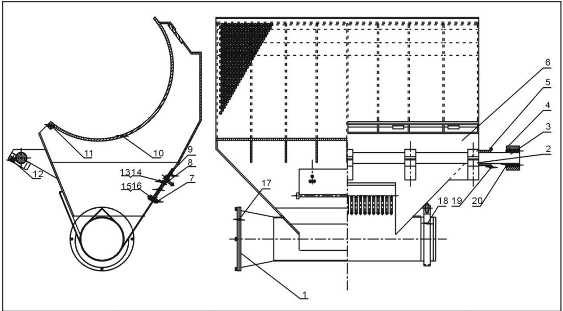
Picture 2-9: Screen Bracket
