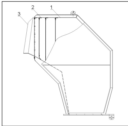
Picture 2-11: Feed-in Box, Material Check Board Inlet
