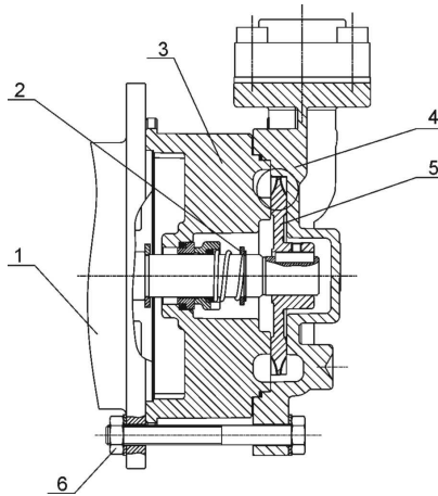
Picture 2-6: Pump
