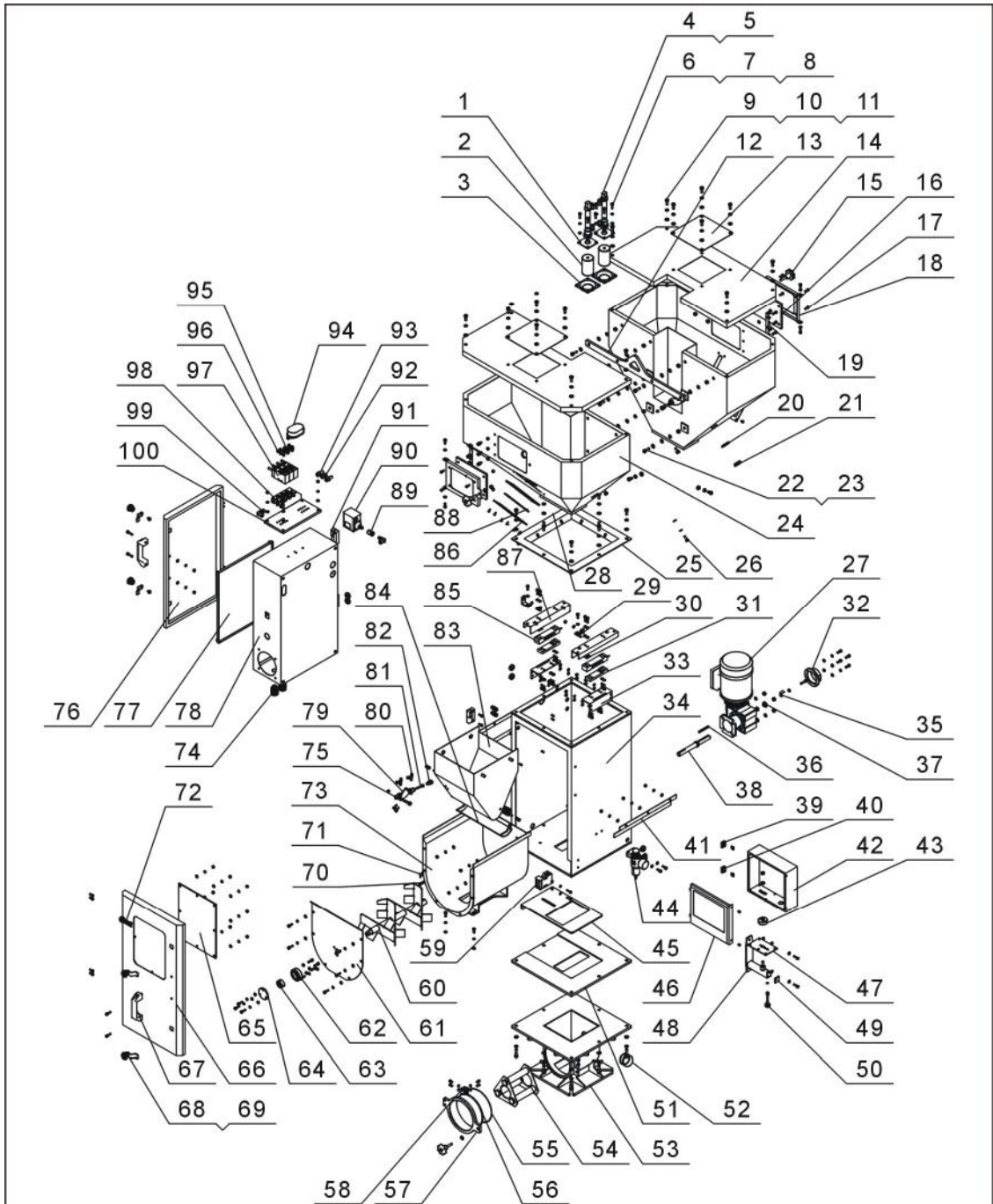
Picture 2-6: SGB-600-2 Assembly Drawing
