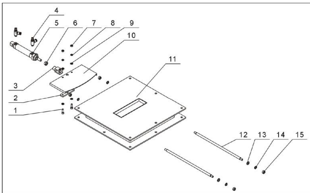
Picture 2-11: Pneumatic Discharge Valve Assembly Drawing
