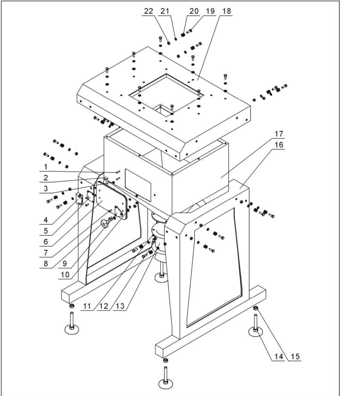
Picture 2-10: Assembly of Floor Stand
