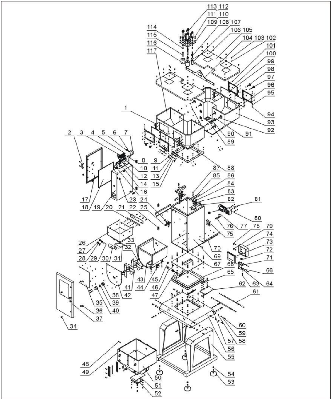
Picture 2-9: SGB-2000-4 Assembly Drawing
