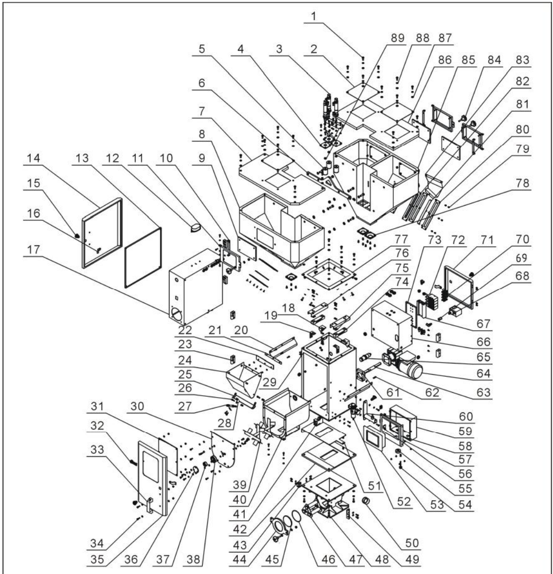
Picture 2-4: SGB-200-3 Assembly Drawing
