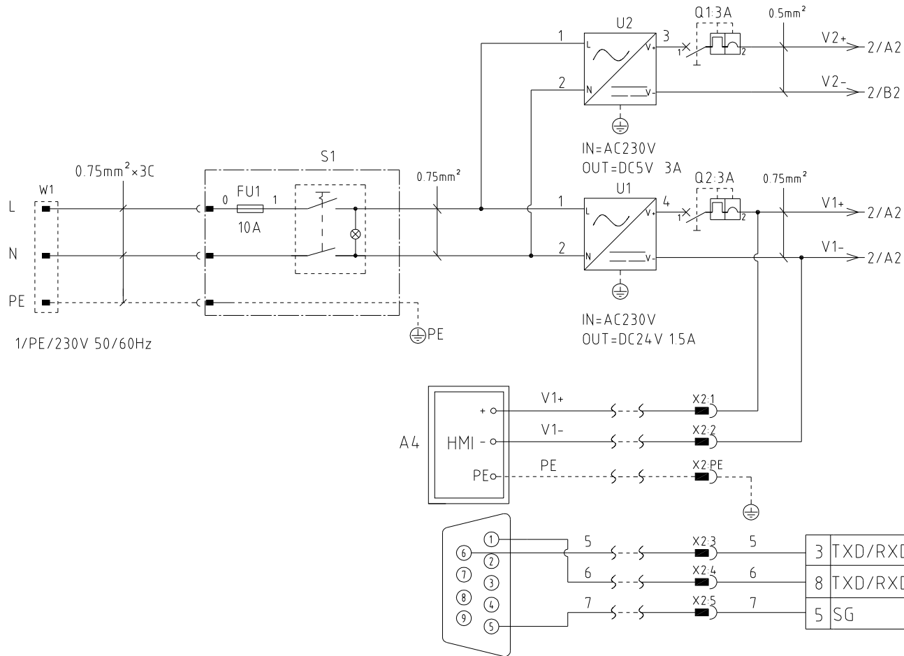
X3 touch panel RS485 comm. wiring diagram
