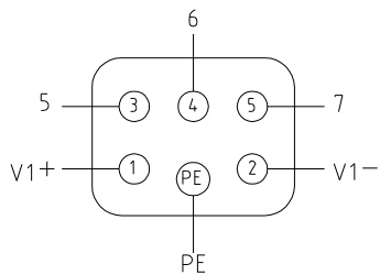
X2 Heavy-duty connector Wiring Diagram
