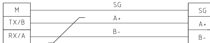
S2 RS485 double communication ports (D-sub 9PIN)
