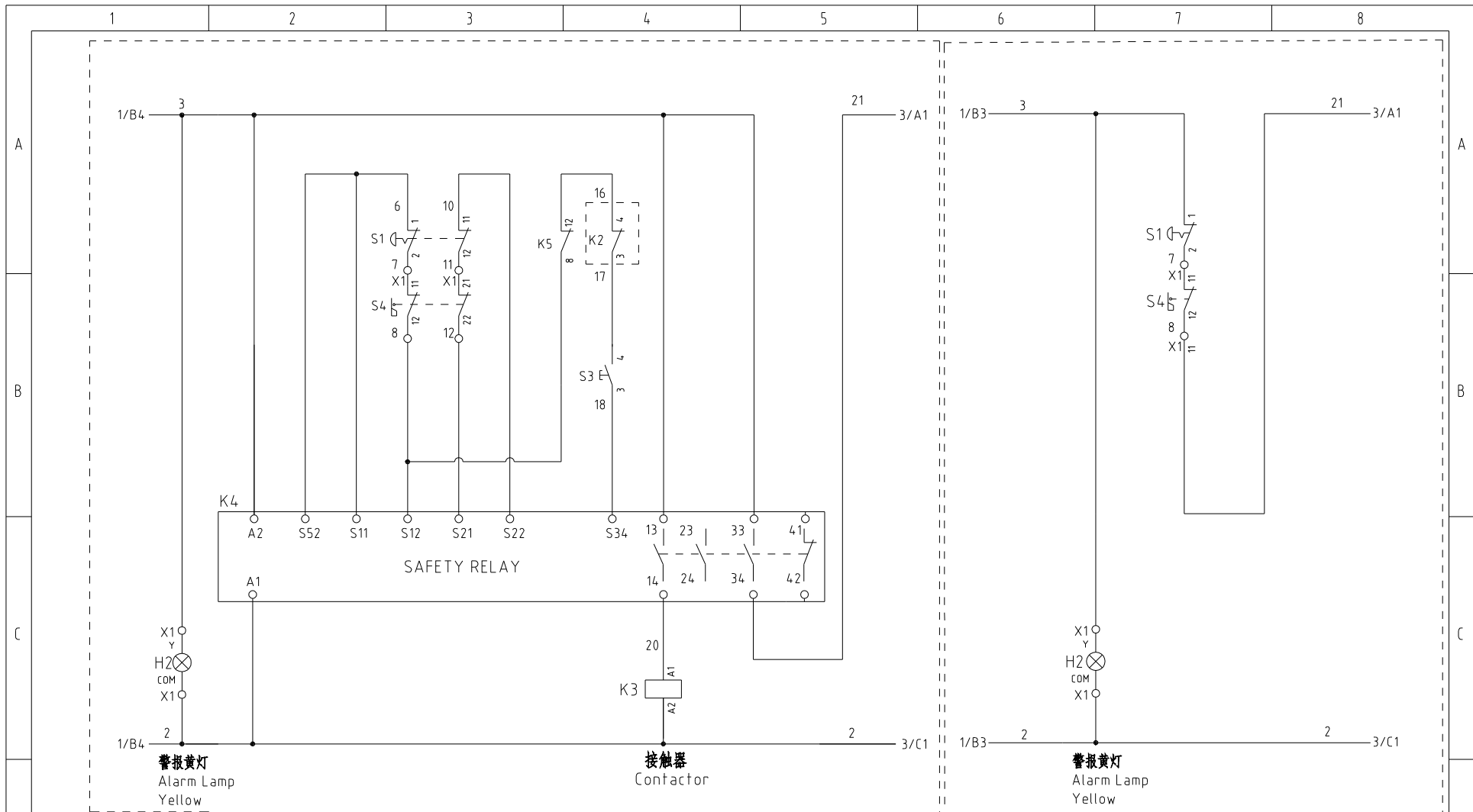
Picture 1 When operation is with optional safety relay
