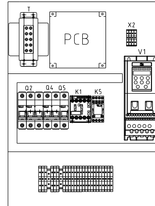
Standard Model Layout 标准机型布局图
