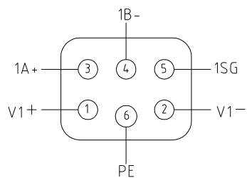
X2 重载接头接线图 X2 Heavy-duty connector Wiring Diagram
