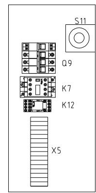
干燥桶2控制箱 Drying hopper 2 Control box
