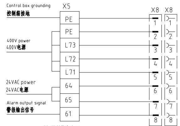
Control box signal of barrel 2 (桶2控制箱内信号)
