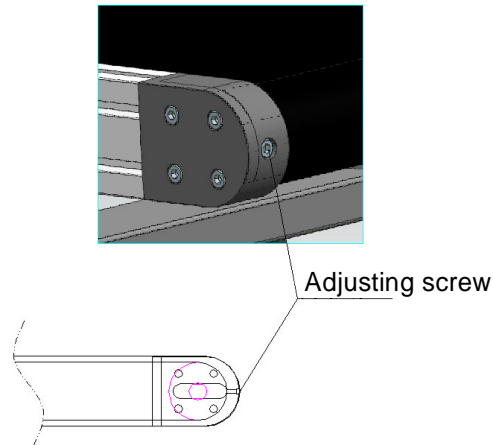
Picture 4-3: Belt Position Adjustment
