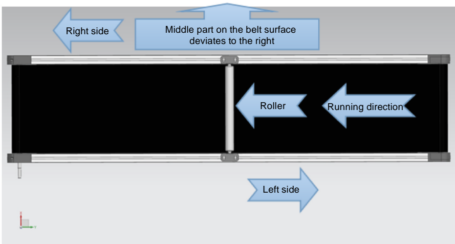
Picture 3-4: Belt Regulation Diagram
