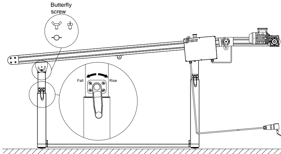
Picture 4-2: Conveyor Adjustment
