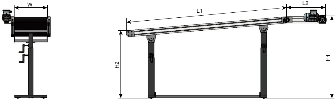
Picture 1-2: SAC Specification
