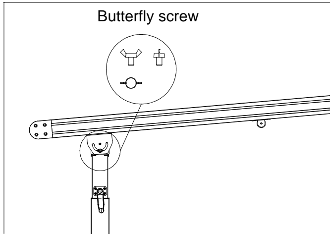
Picture 3-3: Wing Screw Position Diagram
