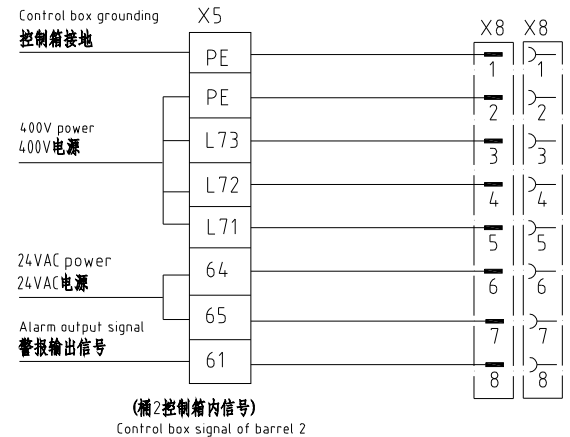
干燥桶2控制箱 Drying hopper 2 Control box
