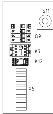
干燥桶2控制箱 Drying hopper 2 Control box
