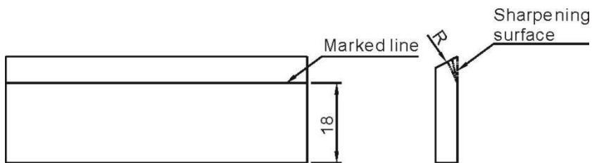
Picture 6-2: Rotating Blades Sharpening
