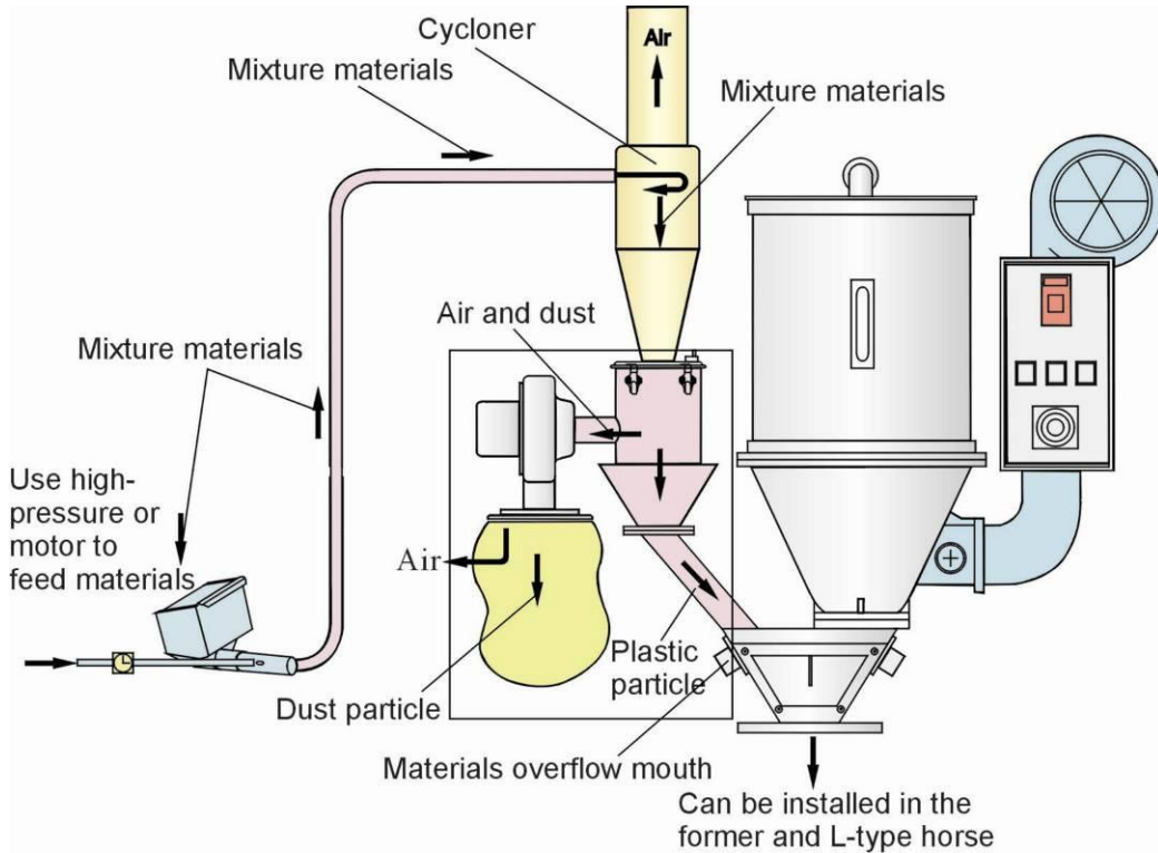
Picture 2-28: Dust Separating System
