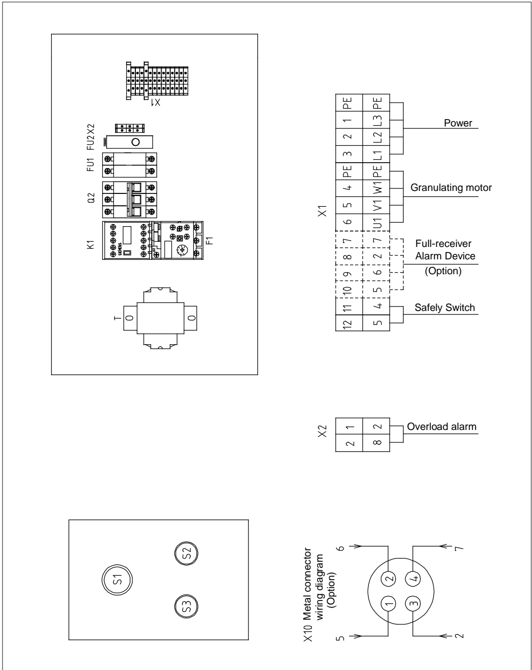
Picture 2-20: Components Layout (400V)
