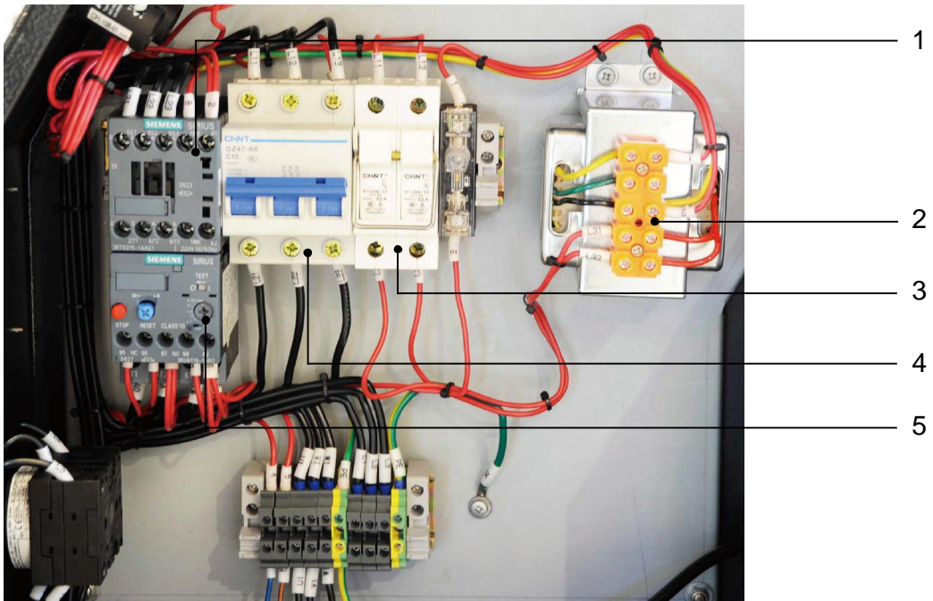
Picture 2-15: Electrical Components Description
