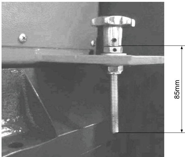
Picture 6-4: Star Screw
