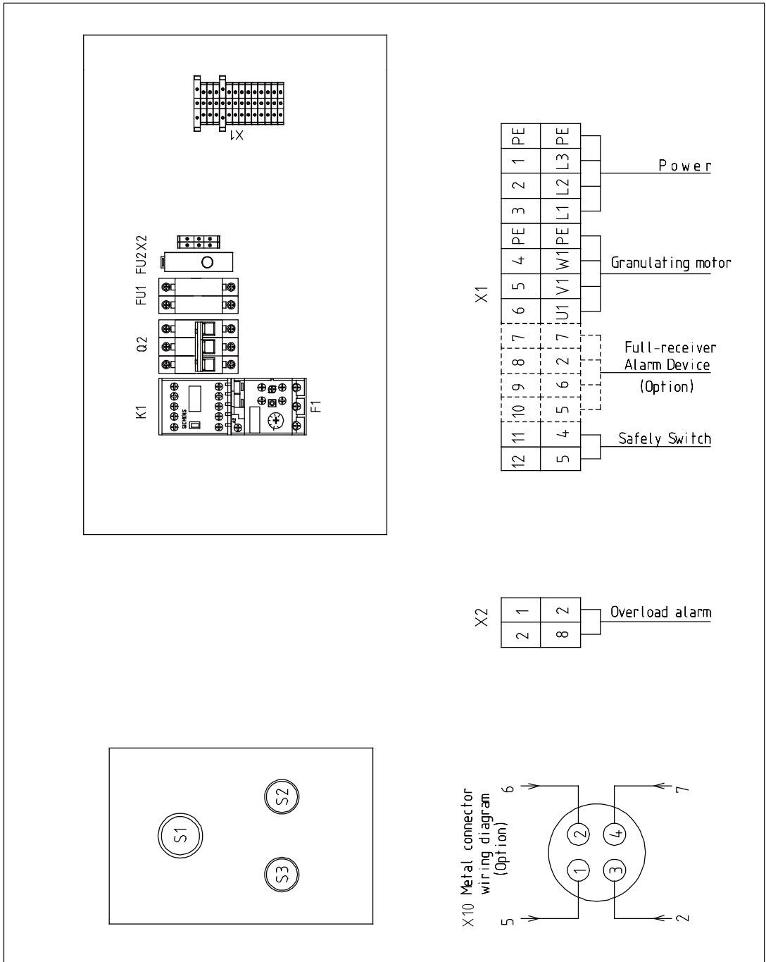
Picture 2-14: Components Layout (230V)
