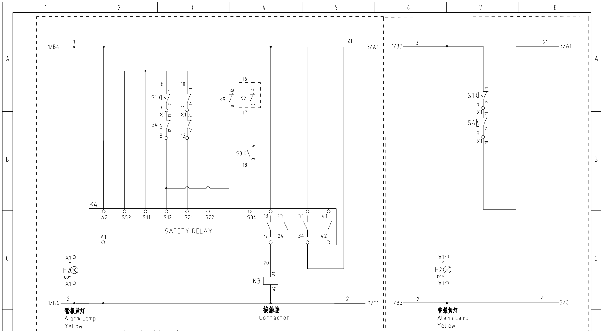
图一当选配安全继电器时使用 Picture 1 When operation is with optional safety relay.
