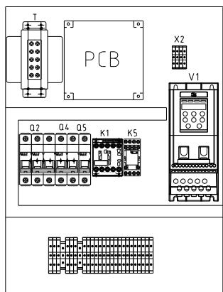
标准机型布局图 Standard Model Layout
