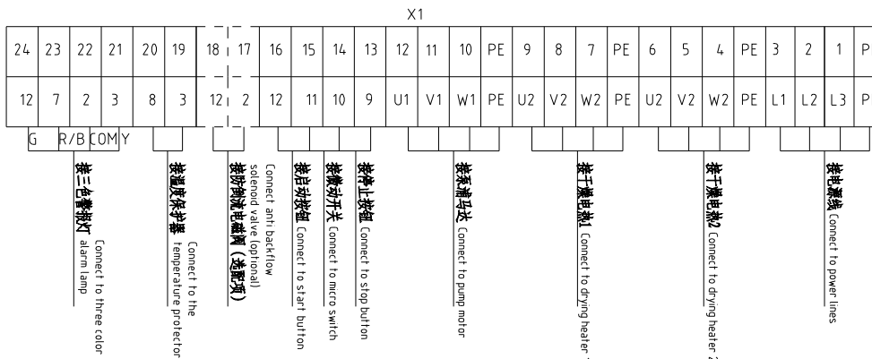
电控箱底板 Base plate of control box
