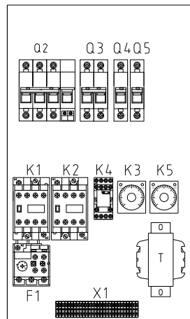
电控箱底板 Base plate of control box
