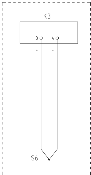
温控表热电偶接线图 Thermocouple wiring diagram for temperature control meter
