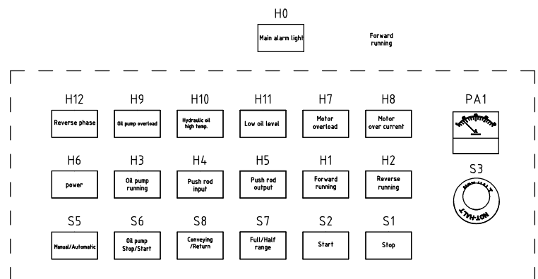
Control Panel Layout
