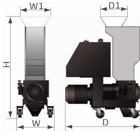
Picture 1-1: Dimensions
