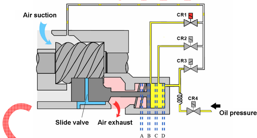
Picture 9-2: Stepless Adjustment Function Sketch
