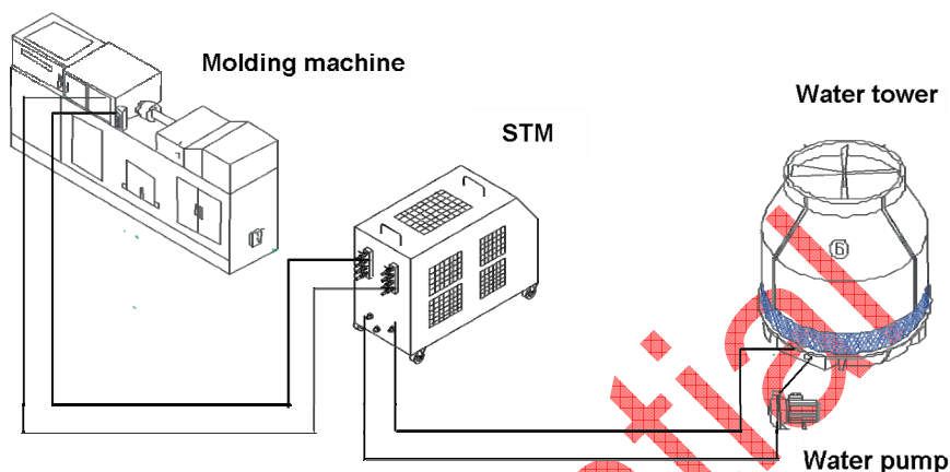
Picture 10-1: Projects Example for STM
