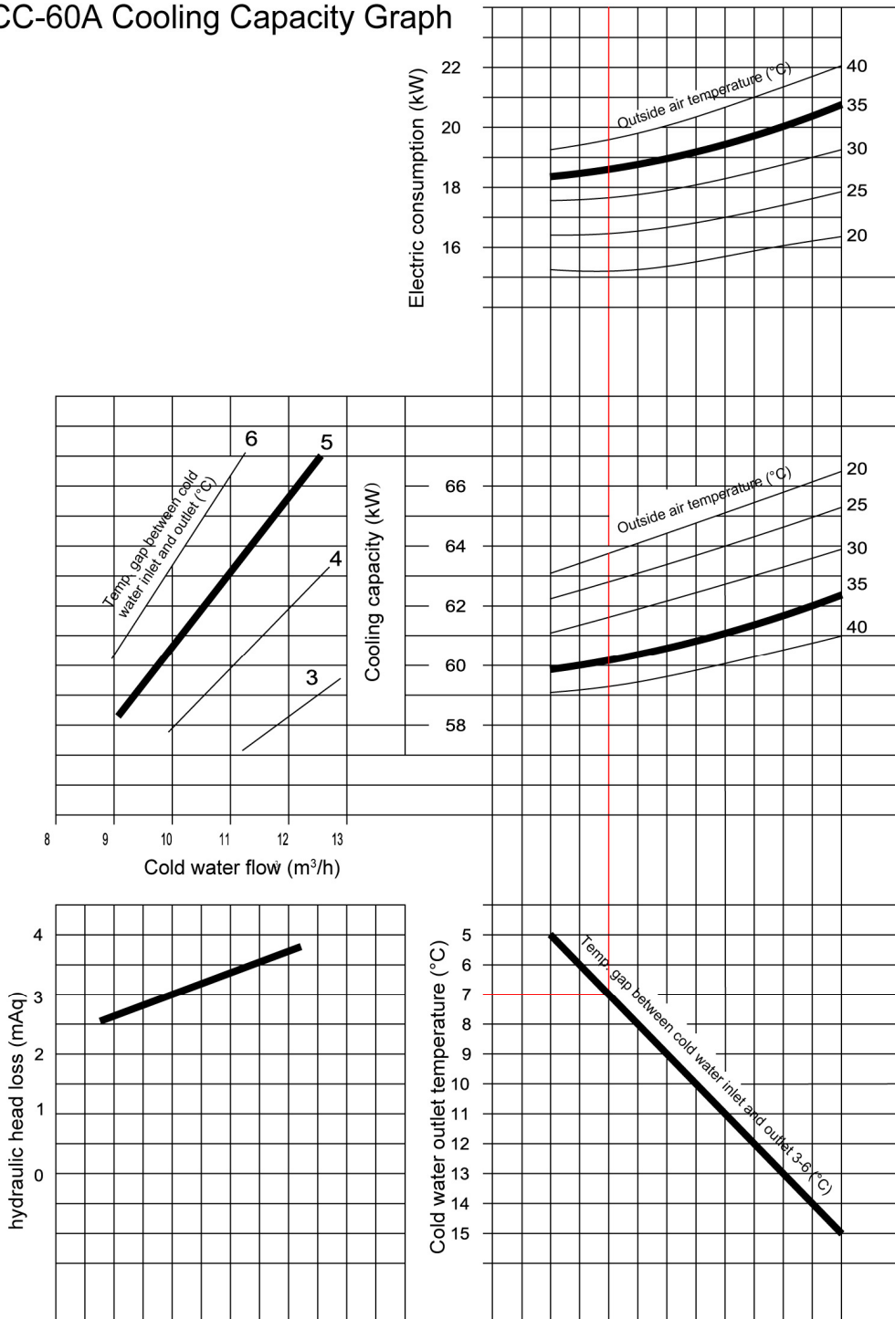
Picture 8-1: SICC-60A Cooling Capacity Graph
