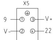
站5重载接头 Station 5 port
