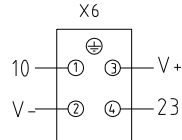
站6重载接头 Station 6 port
