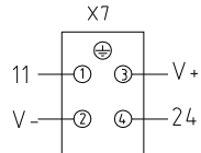
站7重载接头 Station 7 port
