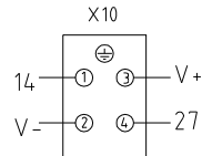
站10重载接头 Station 10 port
