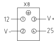
站8重载接头 Station 8 port
