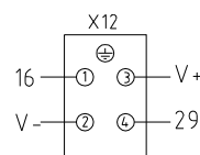
站12重载接头 Station 12 port
