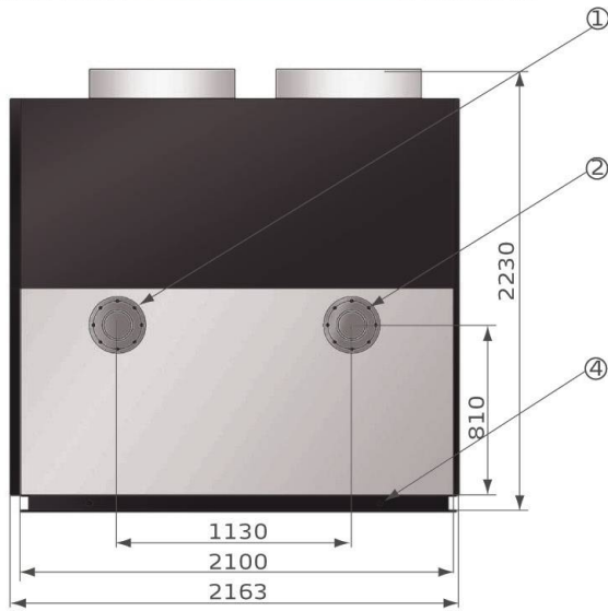
SICC-120A
