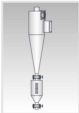
ACF-5"~12"
