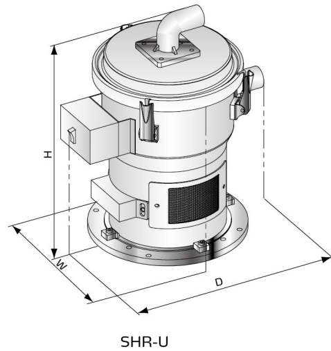
SHR-U
