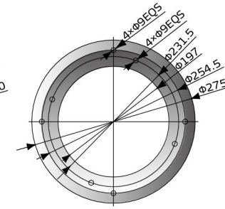
SHR-6U-ST-SHR-24U-ST
