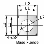
Base Flange
