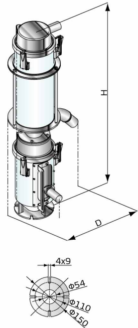
Base Flange
