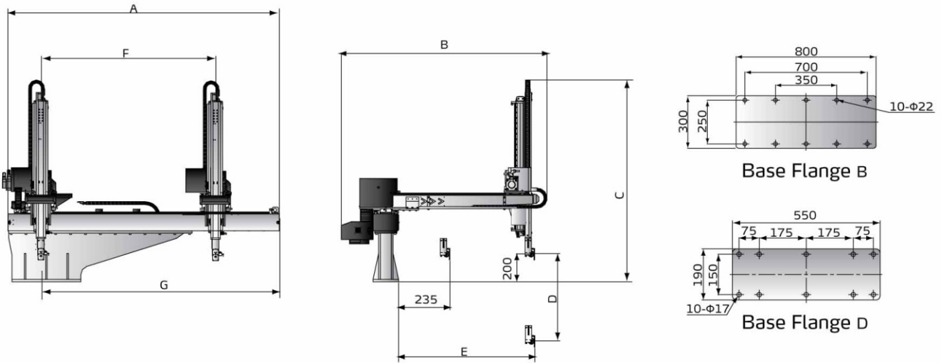
Medium Three Axes Servo Telescopic (Stationary-beam type)
