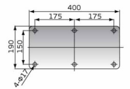
Base Flange C
