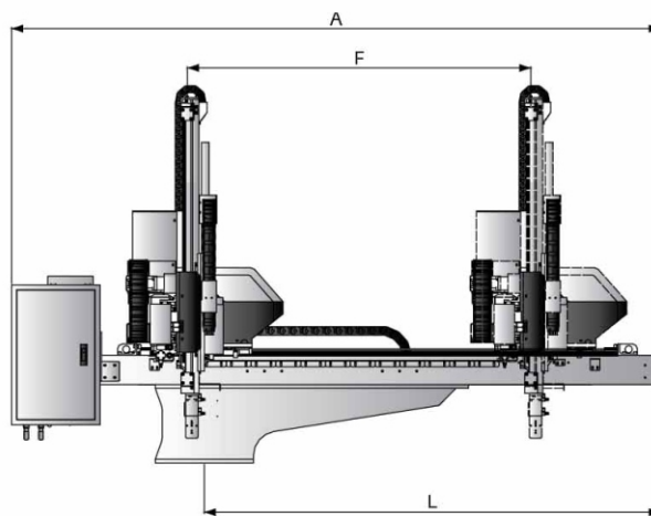
Three Axes Servo Double-arms
