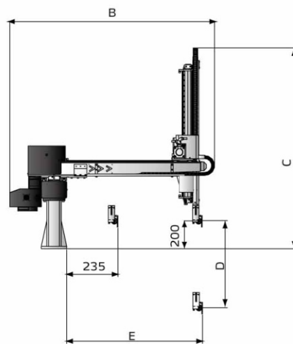
Three Axes Servo Telescopic (Stationary-beam type)
