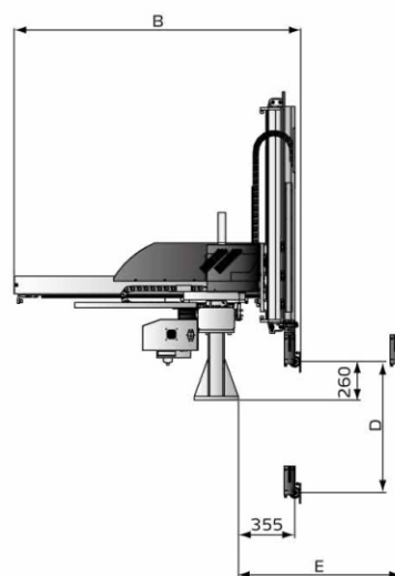
Three Axes Servo Telescopic (Movable-beam Type)
