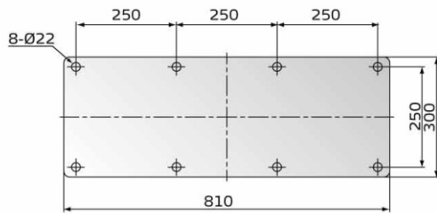
Base Flange
