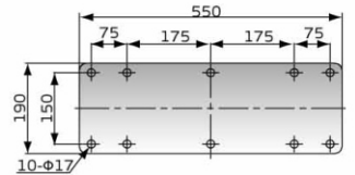
Base Flange D
