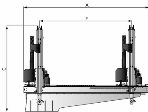
Three Axes Servo Telescopic (Stationary-beam type)
