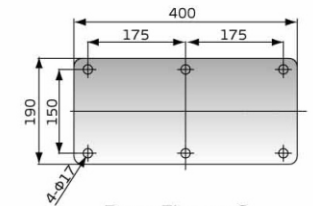
Base Flange C
