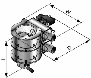
SBU-20/160-D-V
