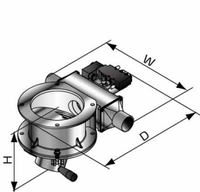
SBU-20/160-S-V
