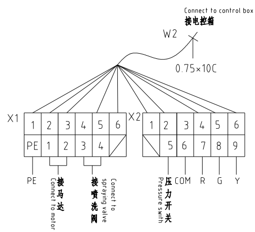
端子排接线图 Terminal block wiring diagram
