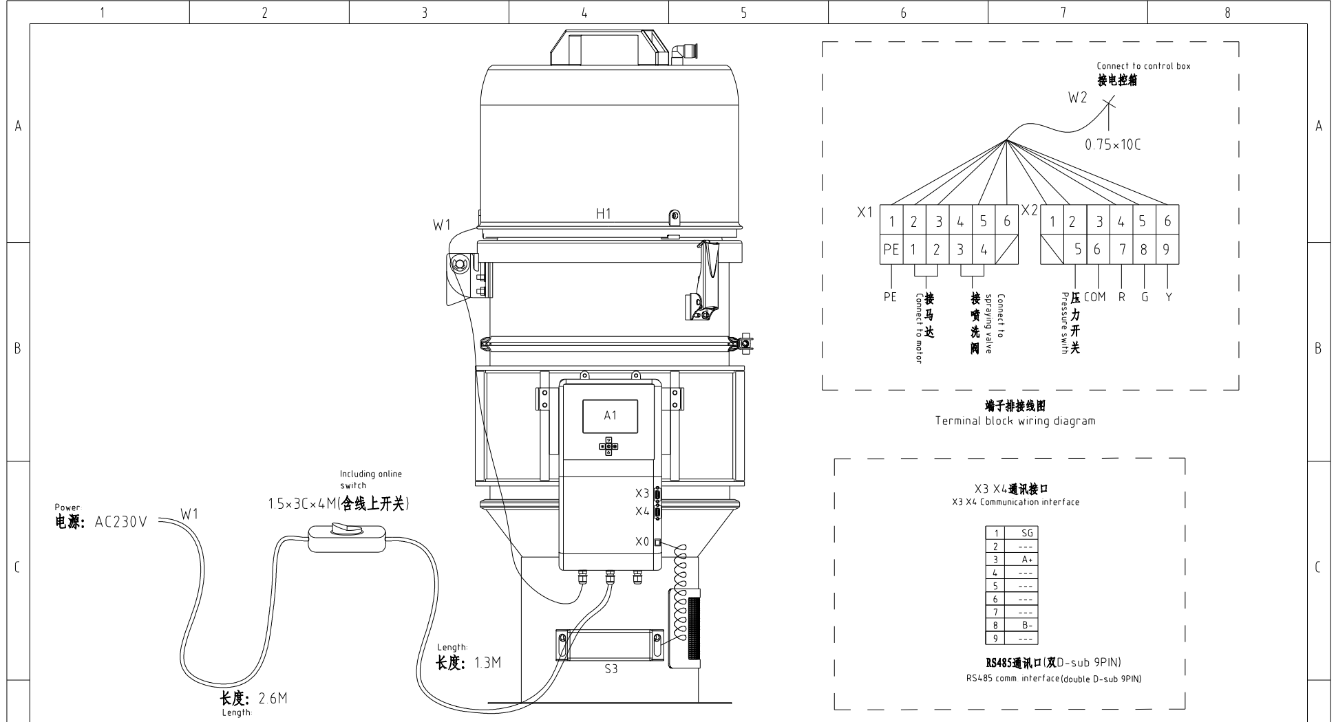
RS485通讯接线图 RS485 Comm. wiring diagram
