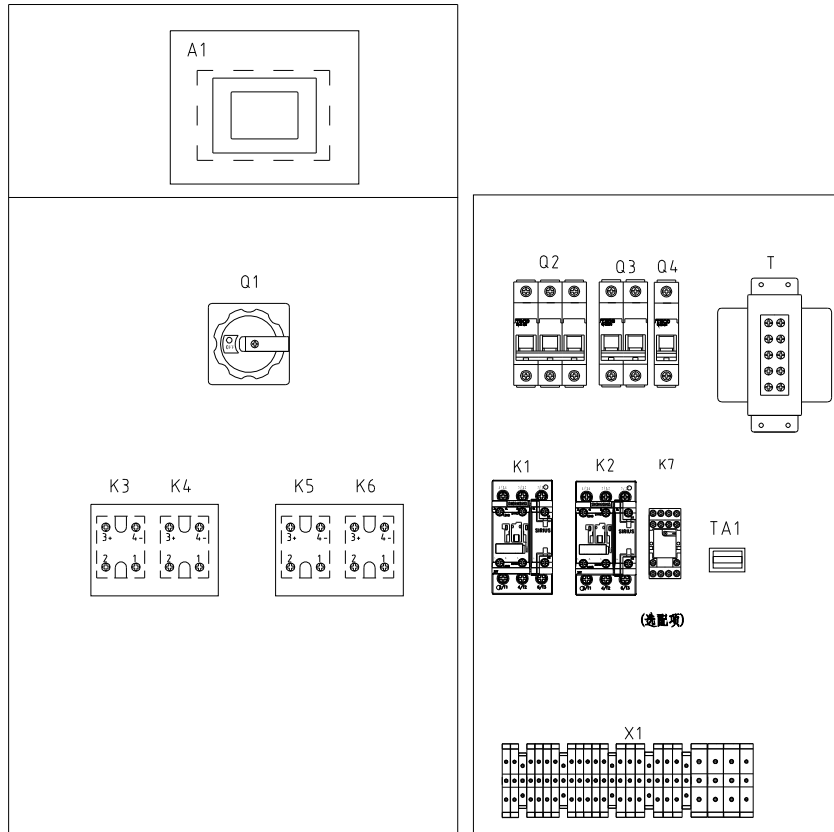
电控外箱 Control box outer case
