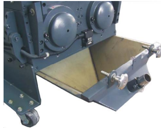
Picture 3-12: Installation of Feed Box, Feed Port and Storage Bin 2
