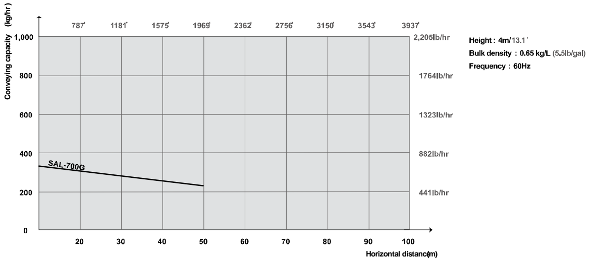
Picture 1-6: Loading Capacity
