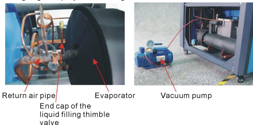
Picture 5-1: Fill in the Refrigerant (1)
