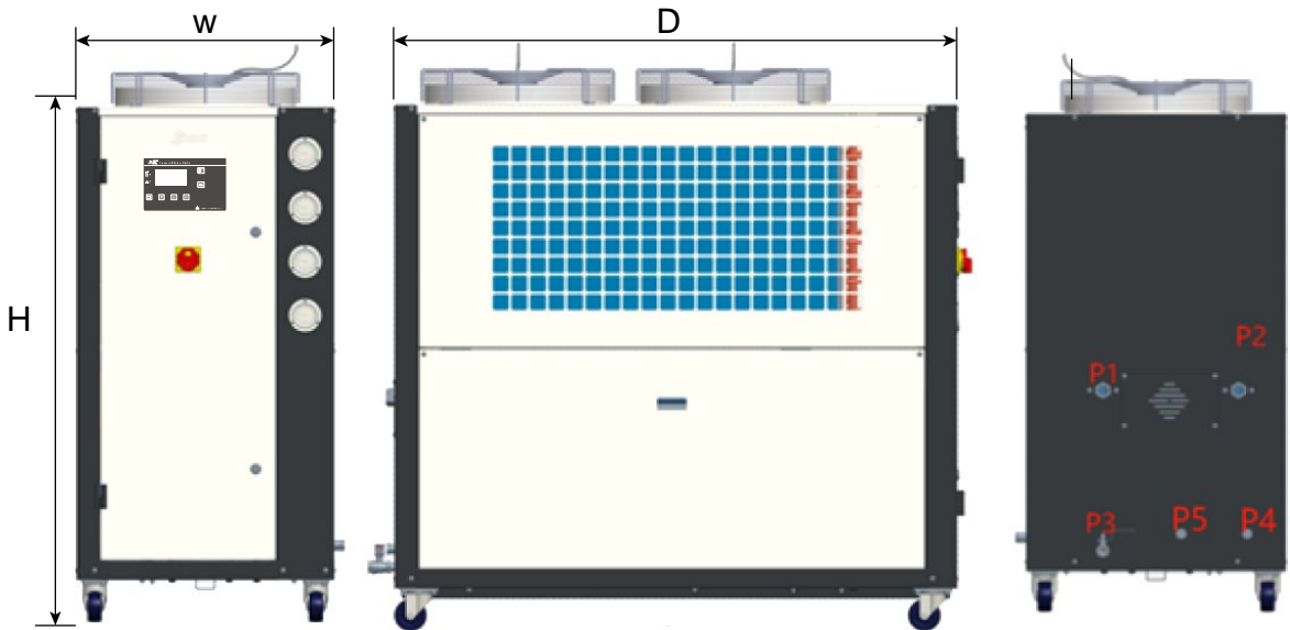
Picture 1-2: Outline Dimensional Drawing
