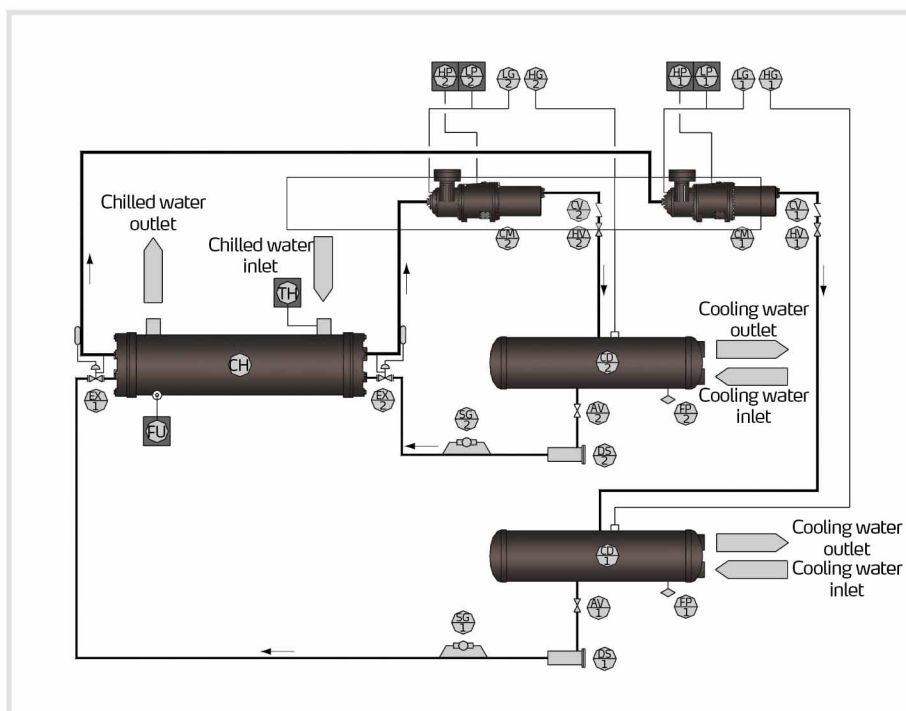
Two Compressors
