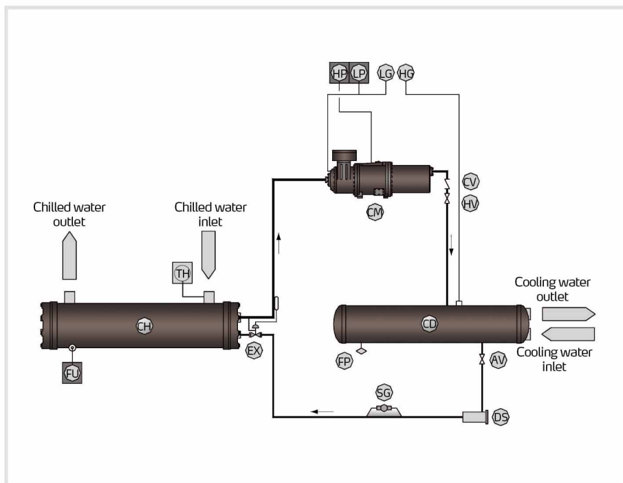
One Compressor
